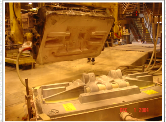
Stripping the Cope Mold off the Pattern
