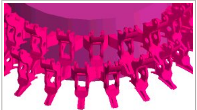
Option B -- Vertical Orientation of Wax Patterns on Sprue
