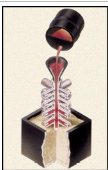
Gravity Casting
