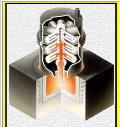
Countergravity Low-Pressure Air (CLA) Investment Casting
