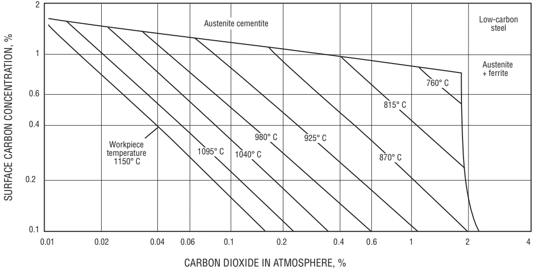
Variation of carbon potential with carbon dioxide concentration for an endothermic-based atmosphere containing 20% CO and 40% H 2 in contact with plain carbon steel at various workpiece temperatures.
