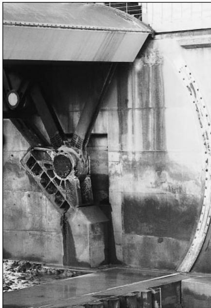
This is a photograph of a sluice gate (open position) on the Thames River Barrier in London. Monel alloy K-500 bolting was used for all the structurals.
