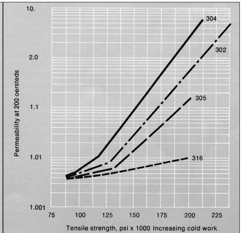
Figure 8 MAGNETIC PERMEABILITY OF AUSTENITIC ALLOYS SUBJECTED TO COLD WORKING CAN ALSO BE EXPRESSED AS A FUNCTION OF TENSILE STRENGTH
