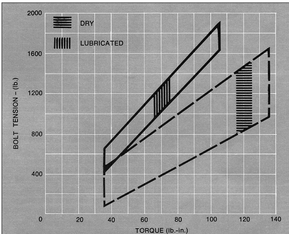
Figure 4 FASTENER LUBRICATION
