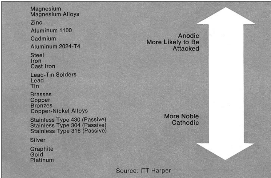
Figure 5 GALVANIC SERIES OF METALS & ALLOYS IN SEAWATER
